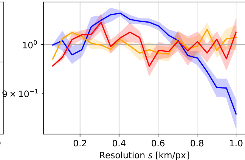
m_2 error [km -2 ]
