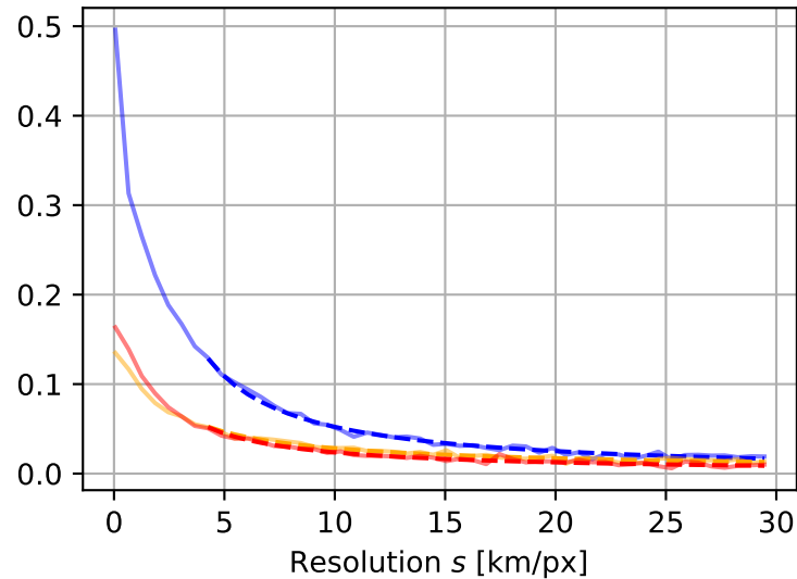
Interface density m_1 [km/km 2 ]
