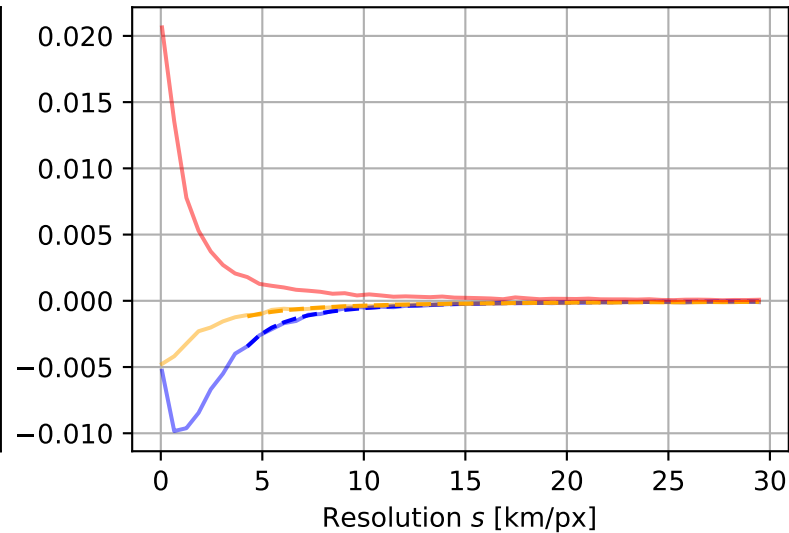
Euler characteristic m_2 [km -2 ]
