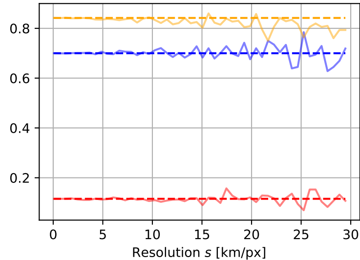
Cloud cover m_0
