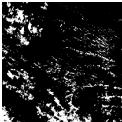
0.42 km/px - (715, 715)
