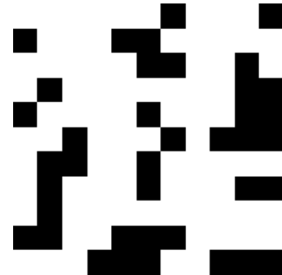
29.94 km/px - (11, 11)
