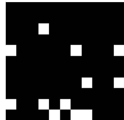
29.94 km/px - (11, 11)
