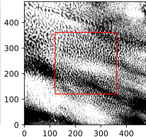
160/256 cl. cover = 0.58
