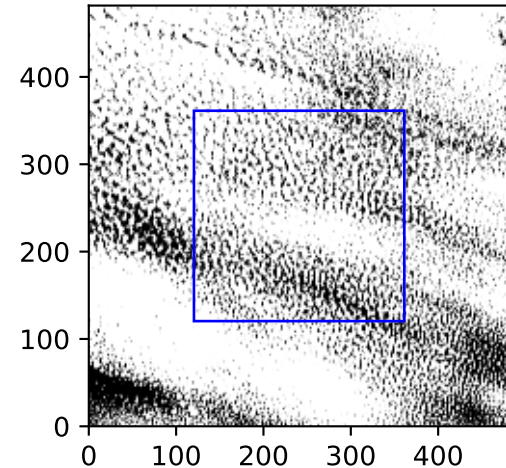
120/256 cl. cover = 0.81
