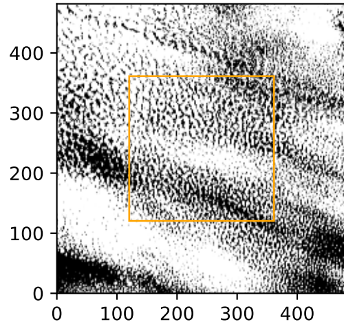
140/256 cl. cover = 0.71
