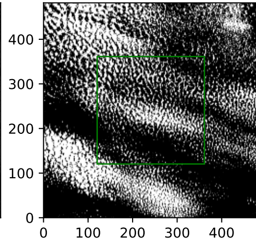
180/256 cl. cover = 0.31
