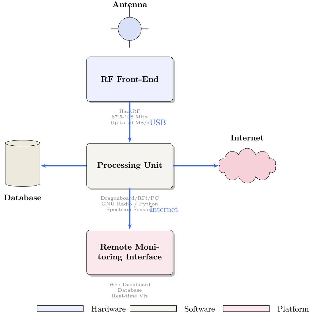
Figure 1: Core Architectural Components
