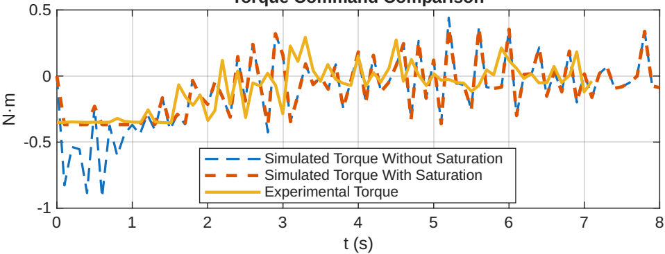
Torque Command Comparison
