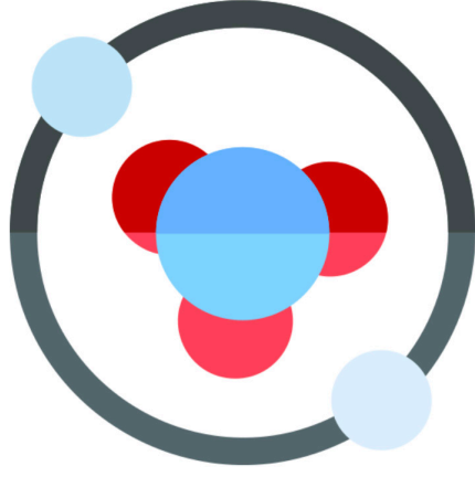
Nucleus
