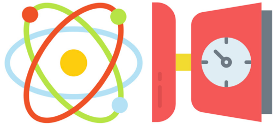
Atomic mass
