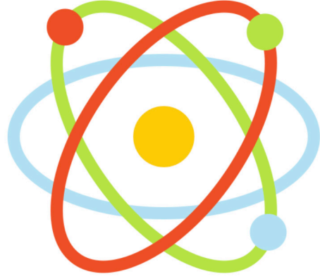
Atom
