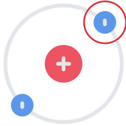
Electrons
