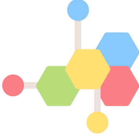
Molecule
