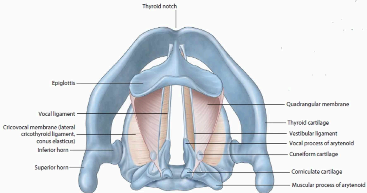
Fibro-elastic membrane of the larynx (superior view)
