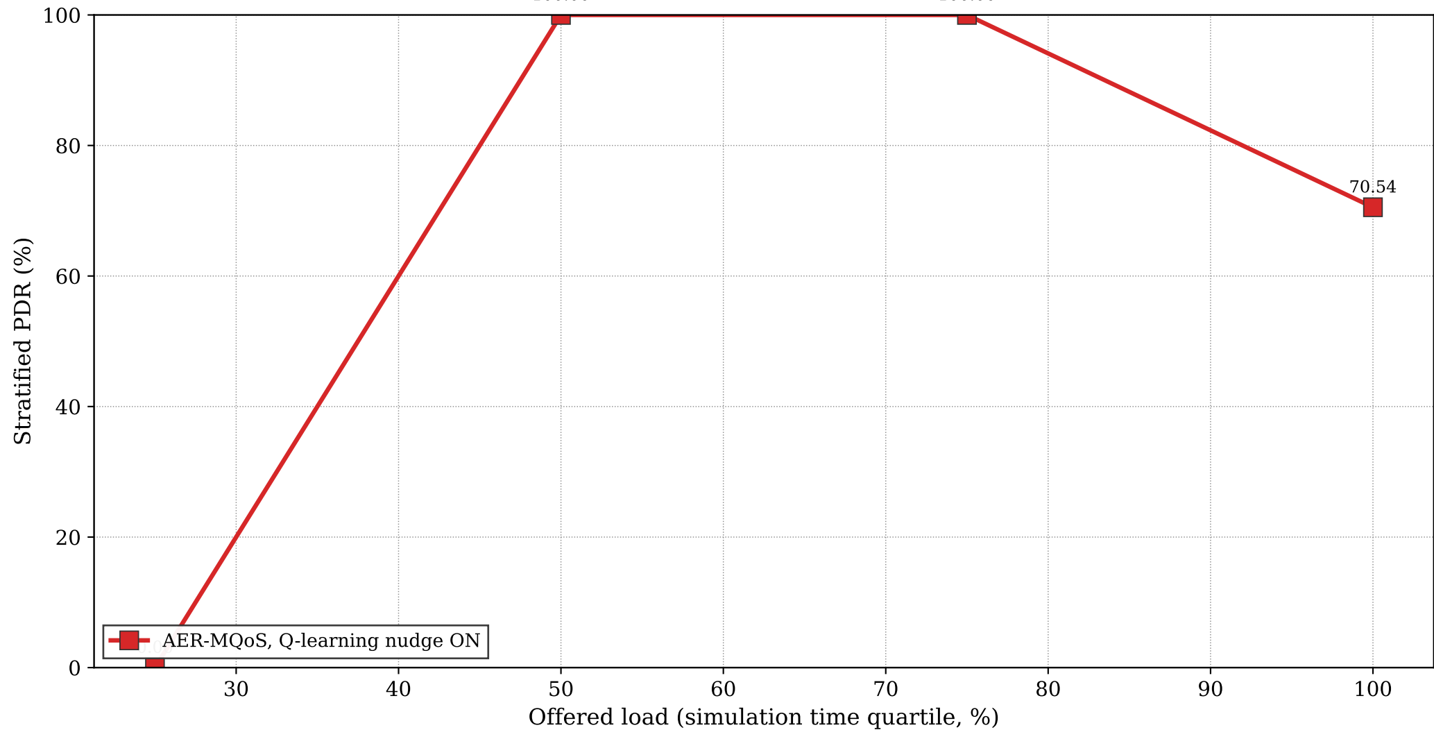
Logging strata: PDR vs. load for AER-MQoS (learning flag in export only)
