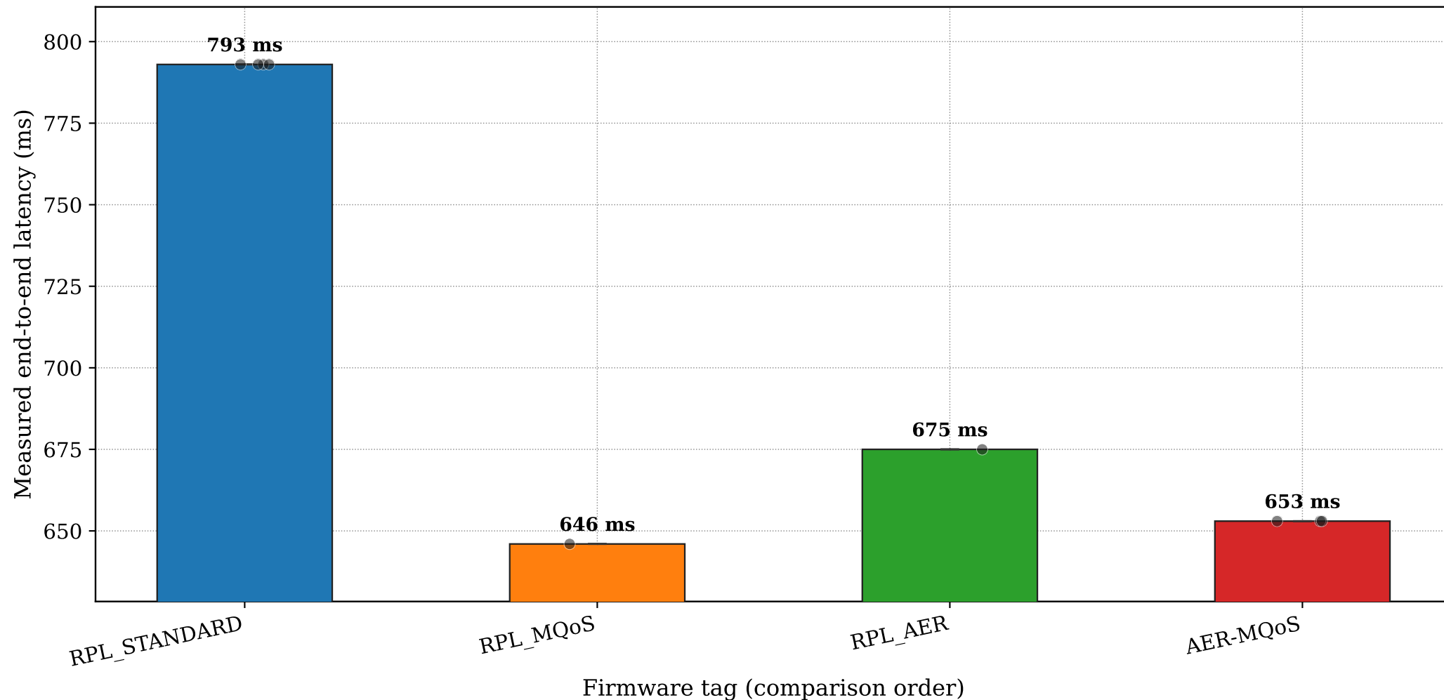
Latency — end-to-end (measured) (lossy UDGGM) (N per Table VII footnotes; \pm\sigma ; dots = individual seeds); campaign summary means (no per-seed variance)
