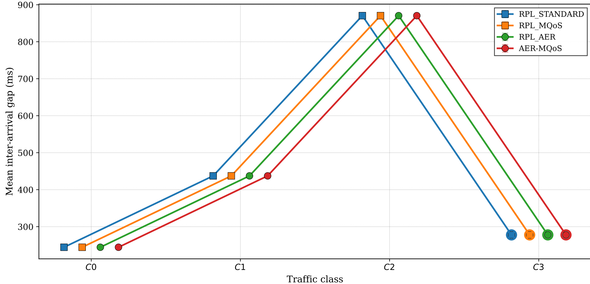
Inter-arrival gap by class (four protocols) (lossy UDM) (not IPDV; per-class C0-C3)
