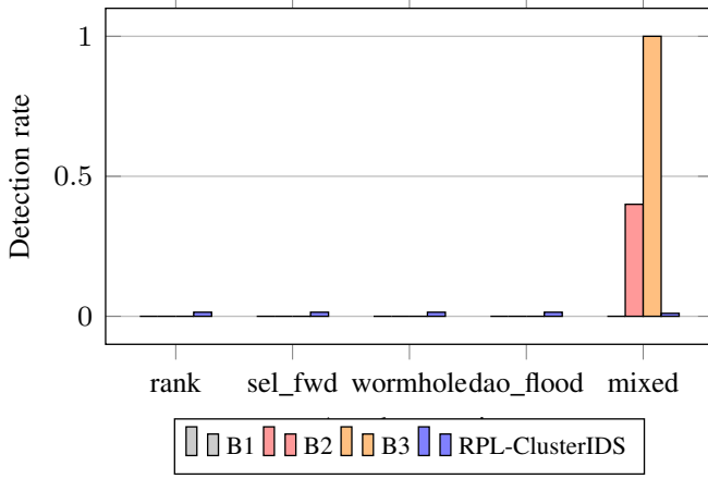
Figure 4. Detection rate across five RPL attack scenarios (50-node grid, BALANCED mode, pilot campaign). RPL-ClusterIDS is compared with centralized rules (B1), flat distributed rules (B2), and centralized verification (B3).
