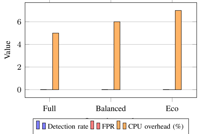
Figure 11. Operating-mode sensitivity (FULL, BALANCED, ECO) for mixed-campaign detection rate, false-positive rate, and member CPU overhead. The policy exposes an explicit security–lifetime trade-off.
