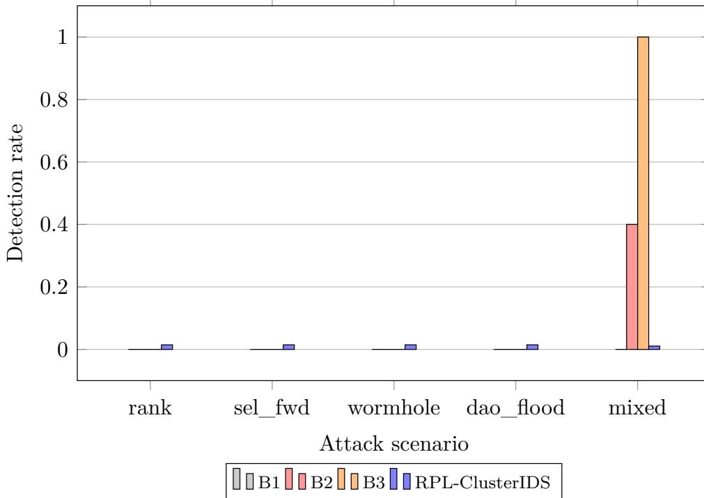
Figure 4: Detection rate across five RPL attack scenarios (50-node grid, BALANCED mode, pilot campaign). RPL-ClusterIDS is compared with centralized rules (B1), flat distributed rules (B2), and centralized verification (B3).
