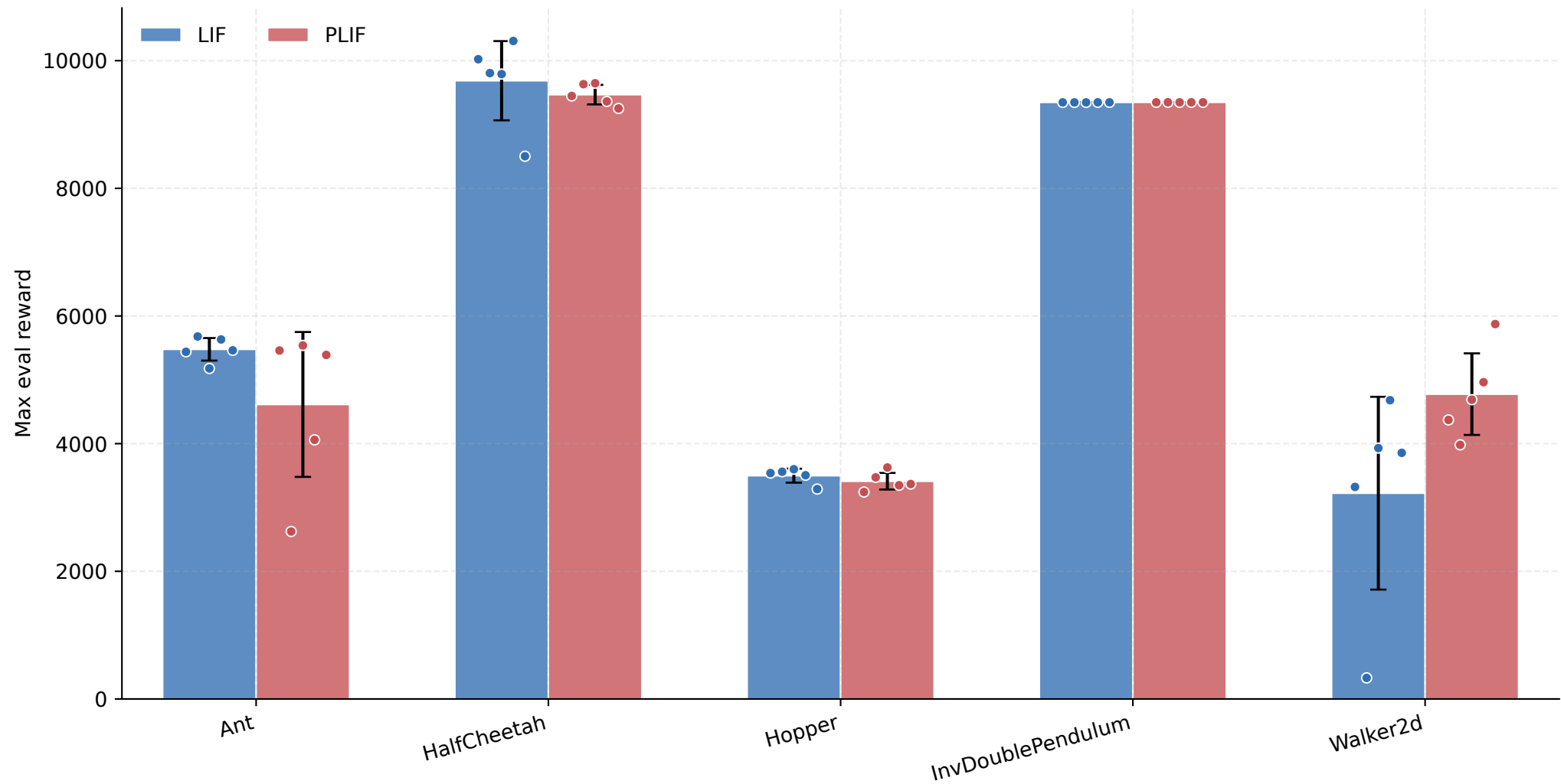
Max Evaluation: LIF vs PLIF
