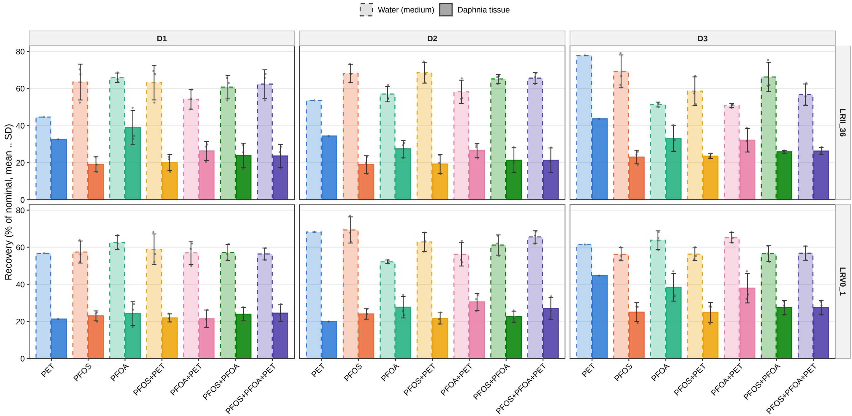
Mass balance: water vs Daphnia tissue by compound and day Mean .. SD; dashed = water, solid = tissue. PFAS: n = 3 per day; PET: n = 1 per day (no error bar)
