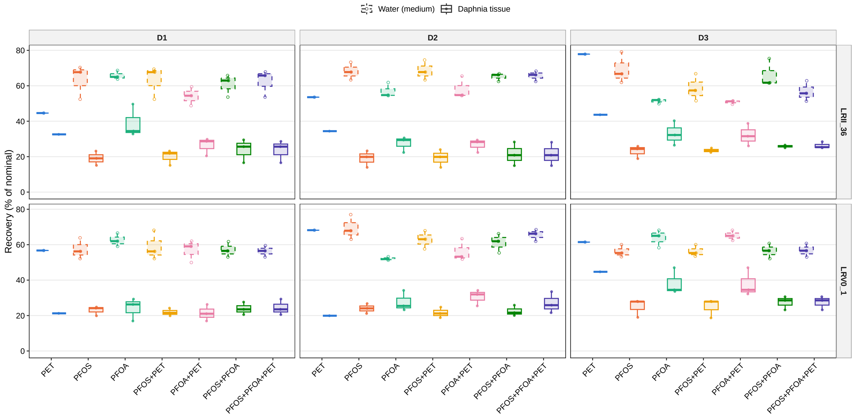
Mass balance: water vs Daphnia tissue by compound and day Dashed = water, solid = tissue. PFAS treatments: 3 replicates per day; PET: 1 value per day
