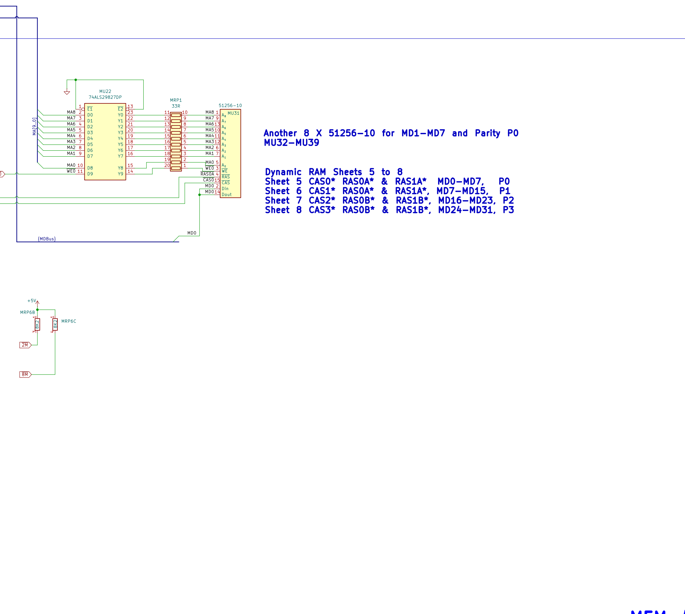
MEM #5 Dynamic RAM sheets 5 to 8 SHEET 5 of 10
