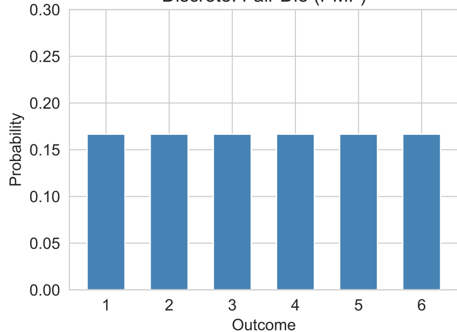
Discrete: Fair Die (PMF)
