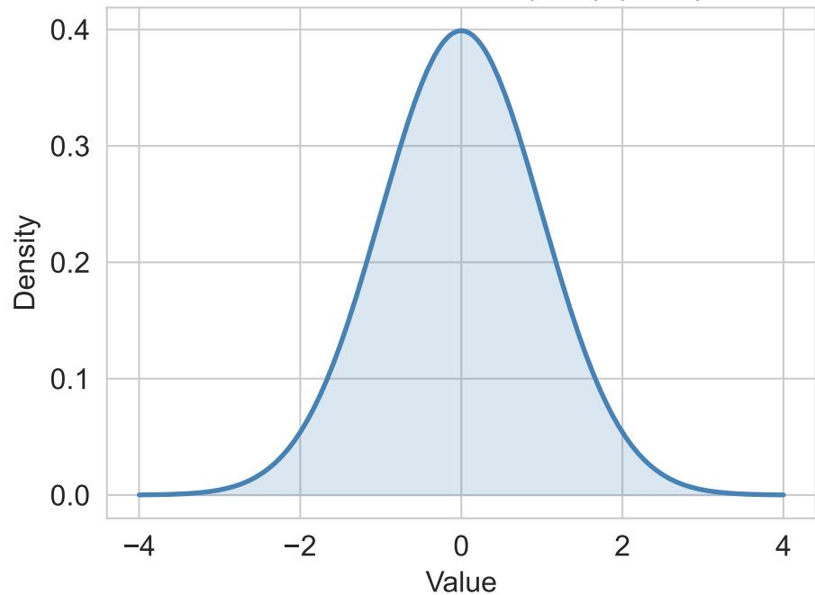
Continuous: Normal(0, 1) (PDF)
