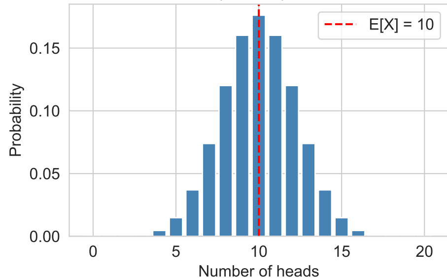
Binomial(20, 0.5): Fair Coin
