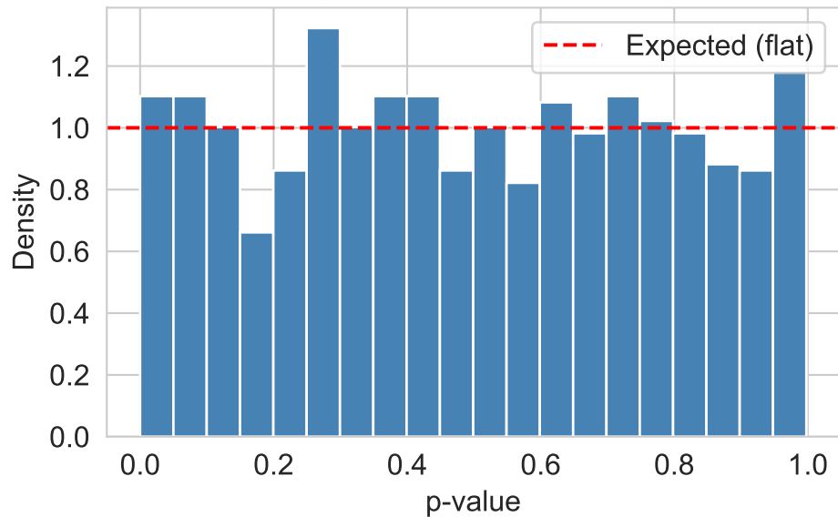
1000 p-values when H_0 is true
