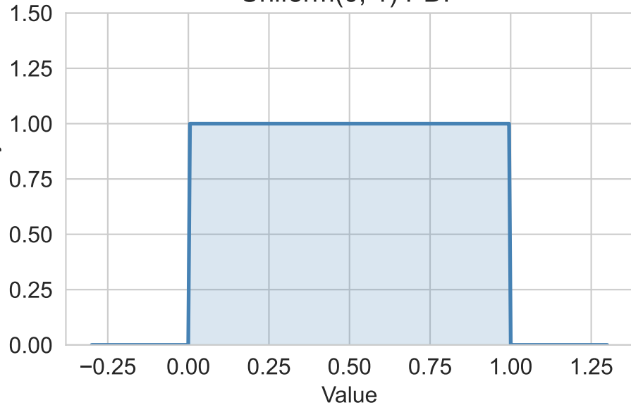
Uniform(0, 1) PDF
