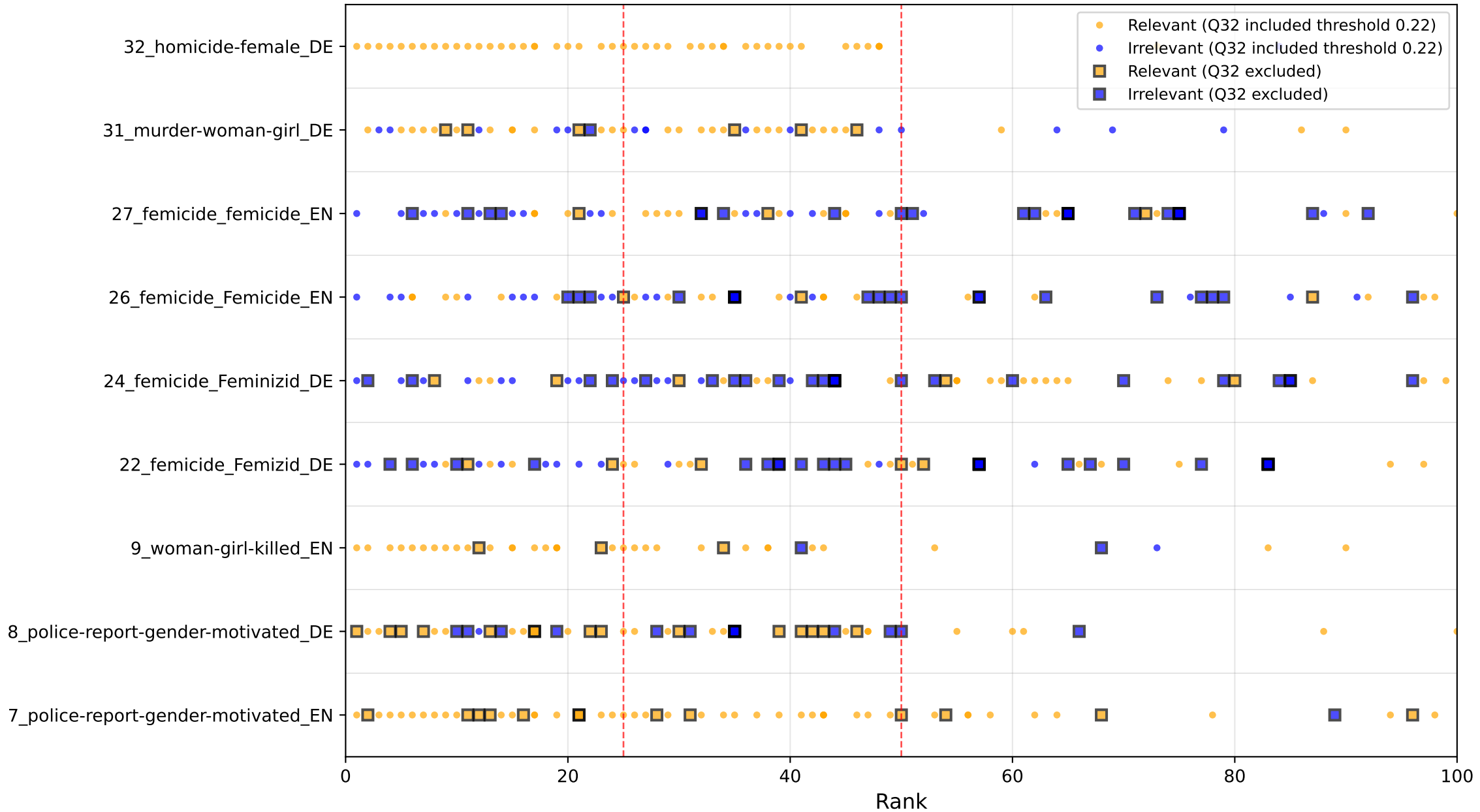
Article Ranks by Query and Relevance, Q32 Threshold 0.22
