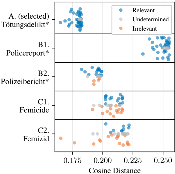
Article Cosine Distance by Query with Relevance
