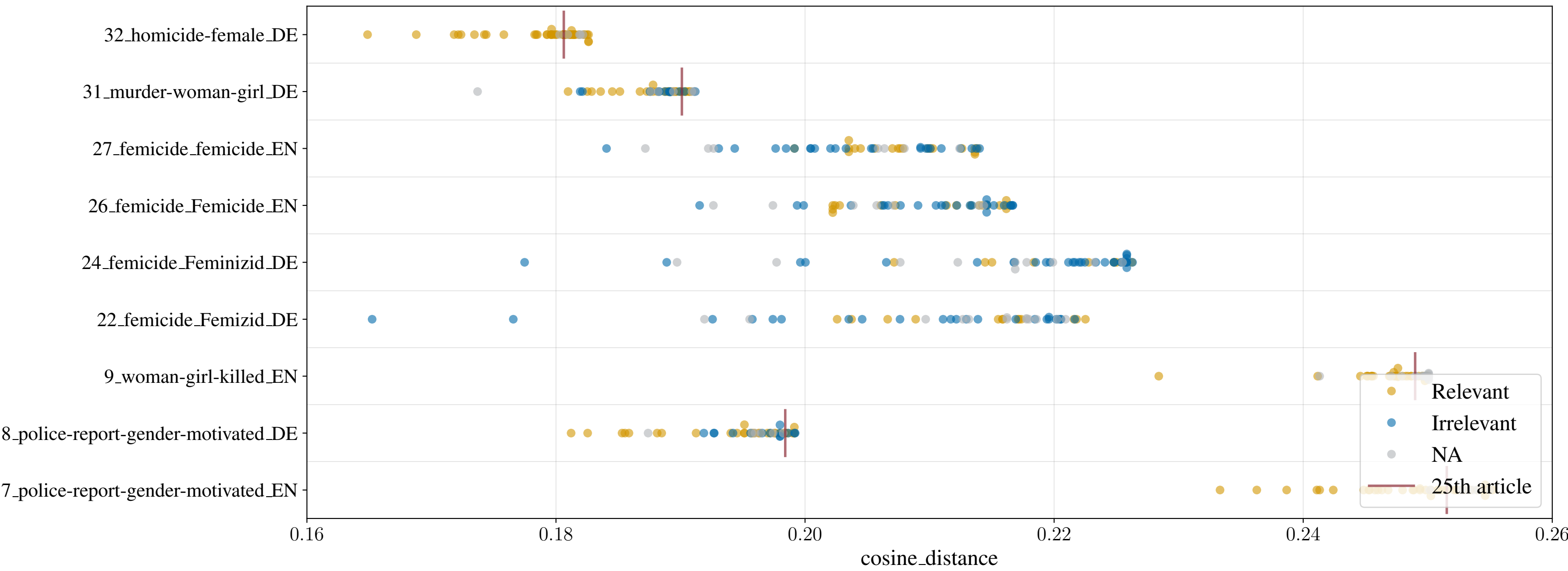
Article cosine_distance by Query with Relevance
