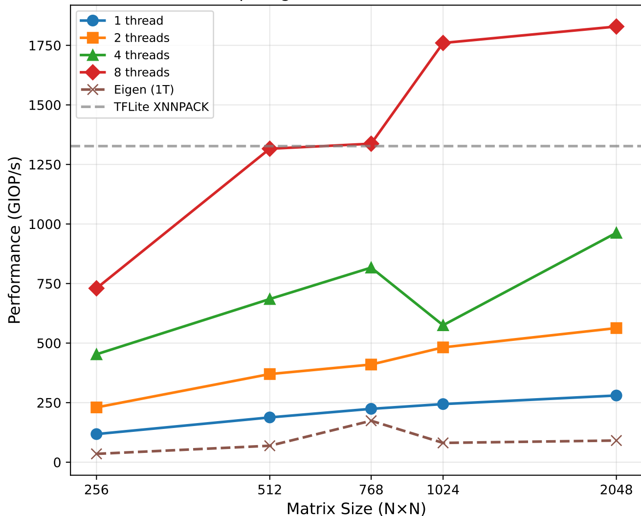
SimpLang INT8 VNNI vs Matrix Size
