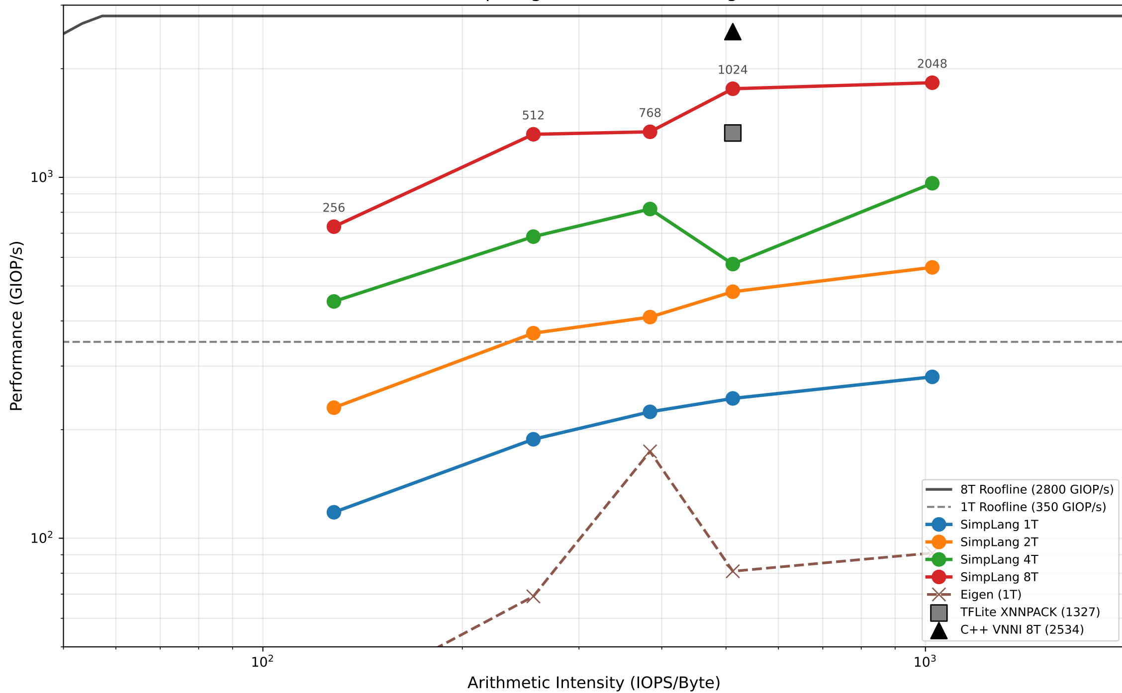
INT8 MatMul Roofline Model SimpLang VNNI Thread Scaling
