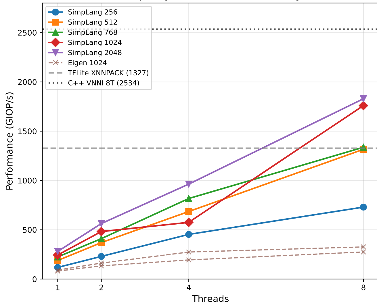
SimpLang INT8 VNNI Thread Scaling
