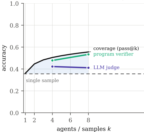
MBPP (headroom +0.20)
