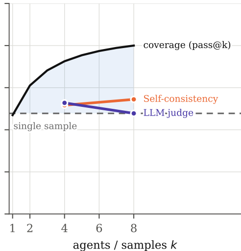
Logic (headroom +0.32)
