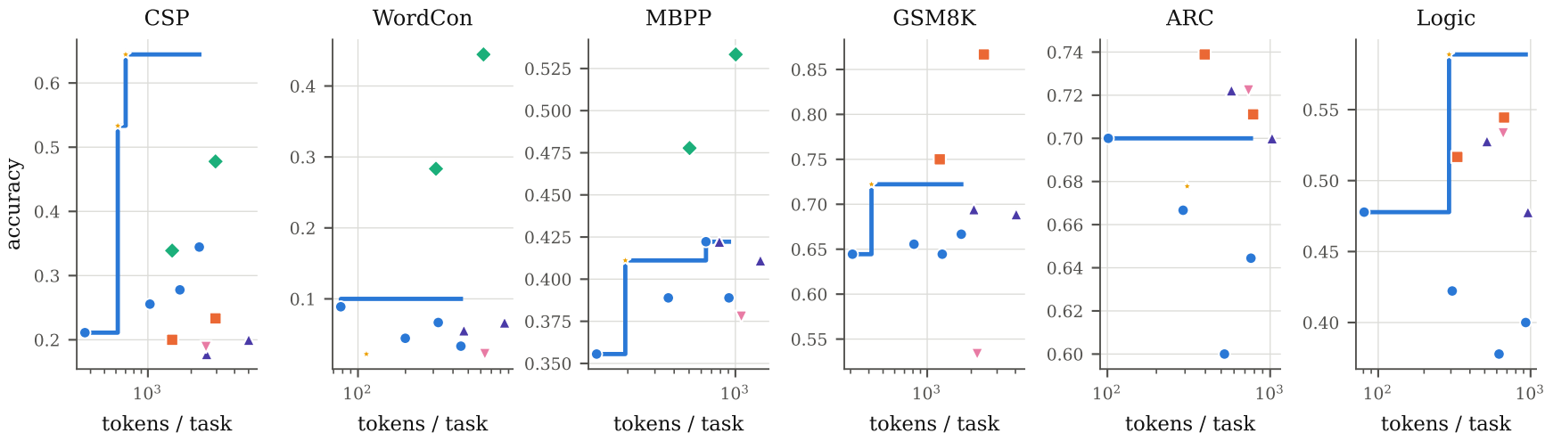
Cost-accuracy frontier, Qwen2.5-1.5B
