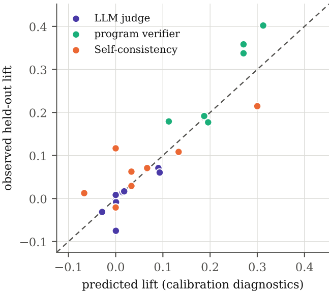
Held-out prediction ( R^2 = 0.84 )
