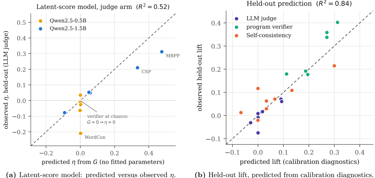
(a) Latent-score model: predicted versus observed \eta . (b) Held-out lift, predicted from calibration diagnostics. Figure 6: Both panels compare against the identity line, not a fitted regression: the theory predicts the value , so a fitted slope would hide bias.
