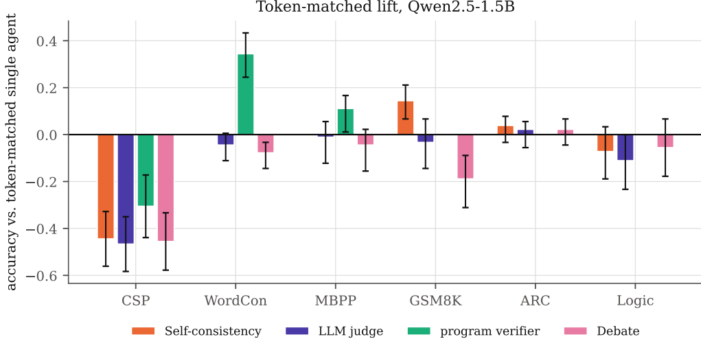
Figure 5: Token-matched lift with 95% cluster-bootstrap intervals, in which both the multi-agent accuracy and the single-agent frontier are recomputed inside every resample.
