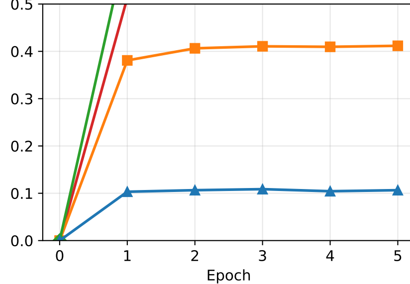
Mean Binary Faithfulness (flip rate)
