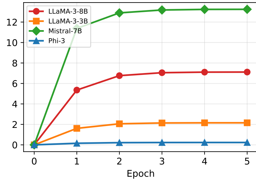
Mean Efficacy (CoT step prob drop)
