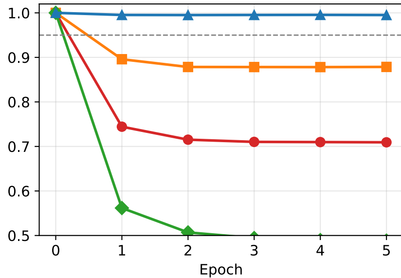
Mean Specificity
