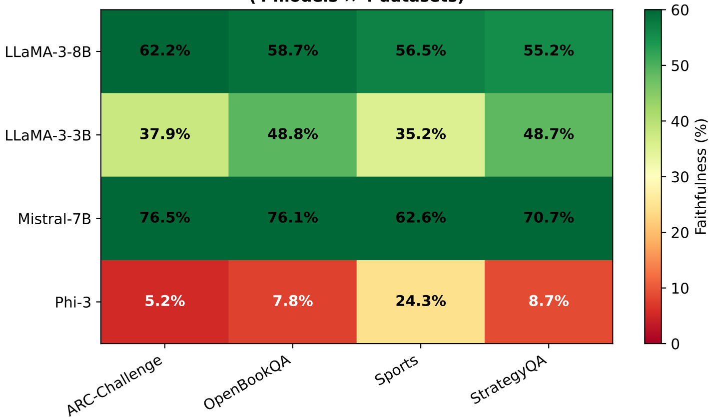
Parametric Faithfulness (%) — NPO Baseline (4 models × 4 datasets)
