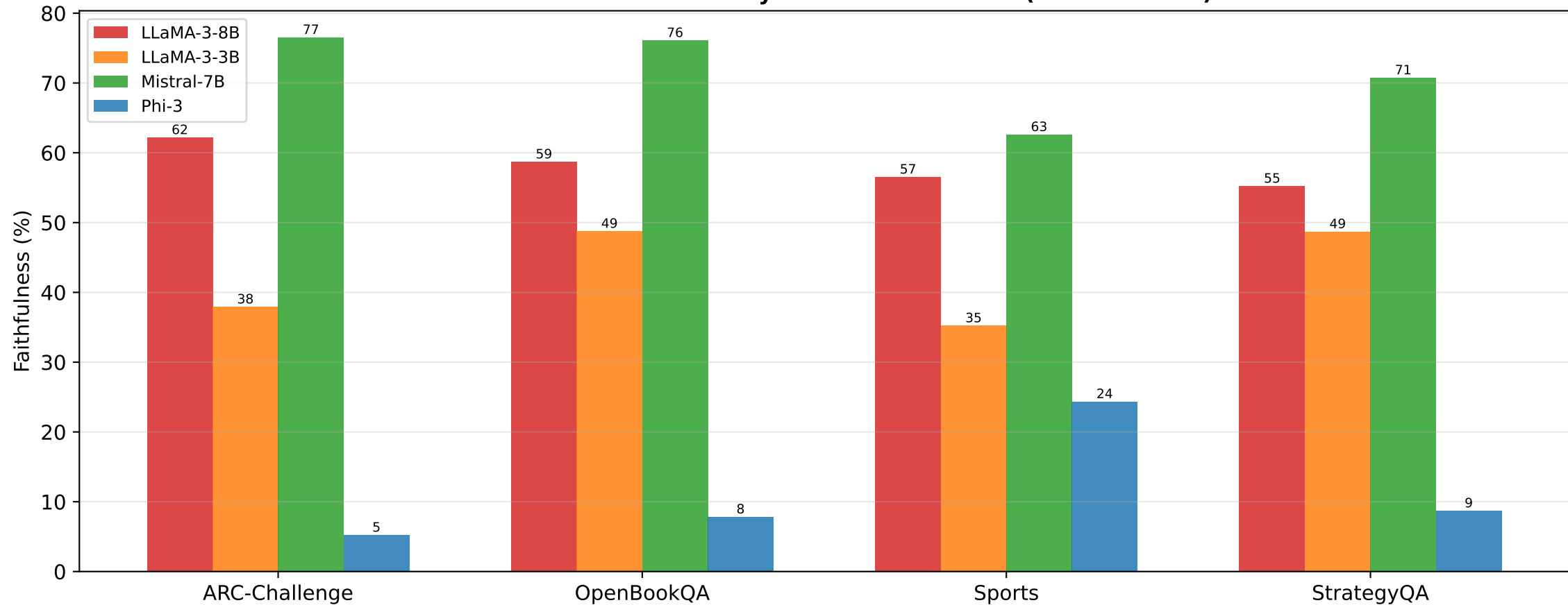
Parametric Faithfulness by Dataset and Model (NPO Baseline)
