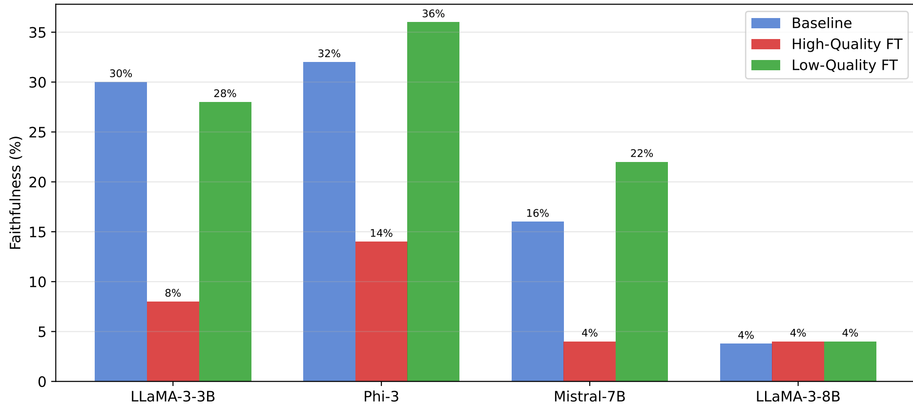
Faithfulness Across All Fine-Tuning Conditions (All 4 Models)
