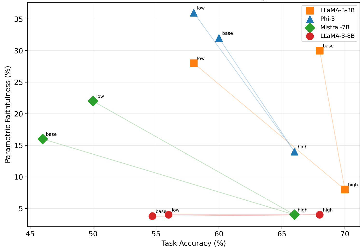
Accuracy vs Faithfulness Tradeoff (arrows show effect of fine-tuning)
