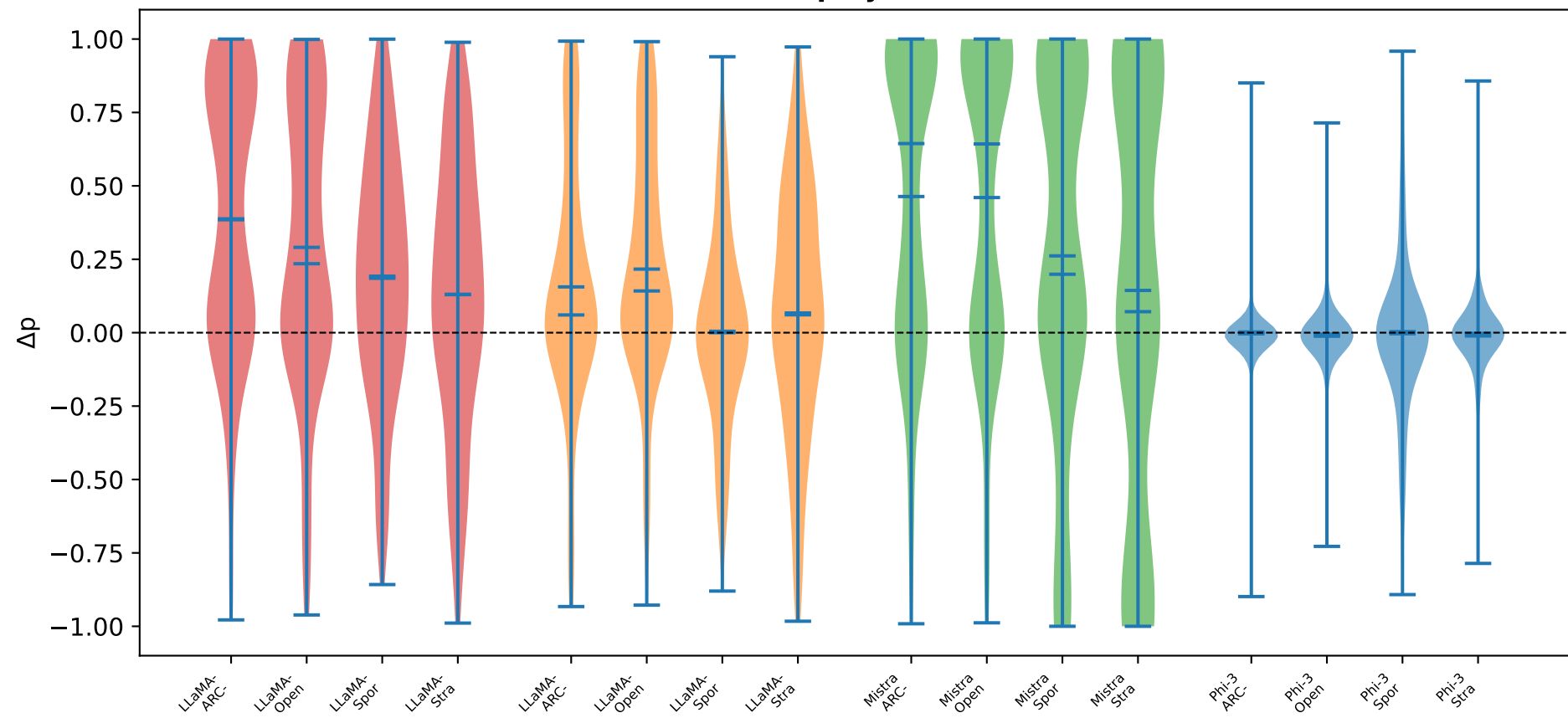
Distribution of \Delta p by Model \times Dataset
