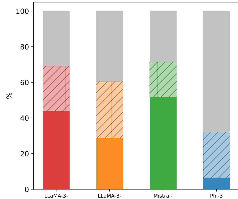
(F) Subcritical
