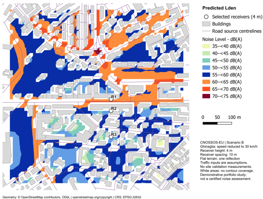
Figure 1. Predicted Lden in dB(A) at 4 m height. A: baseline. B: Ghinaglia speeds reduced from 50 to 30 km/h. Grey polygons are buildings, purple lines road centrelines, and white circles the three selected receivers. White gaps have no contour coverage. Geometry © OpenStreetMap contributors, ODbL. EPSG:32632.
