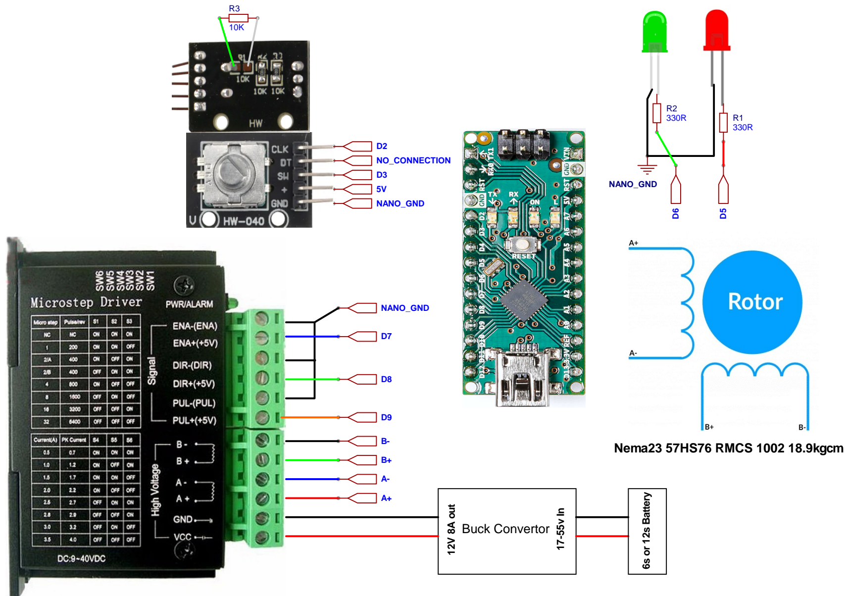
DSR STEPPER MOTOR CONTROL (Prototype v1)
