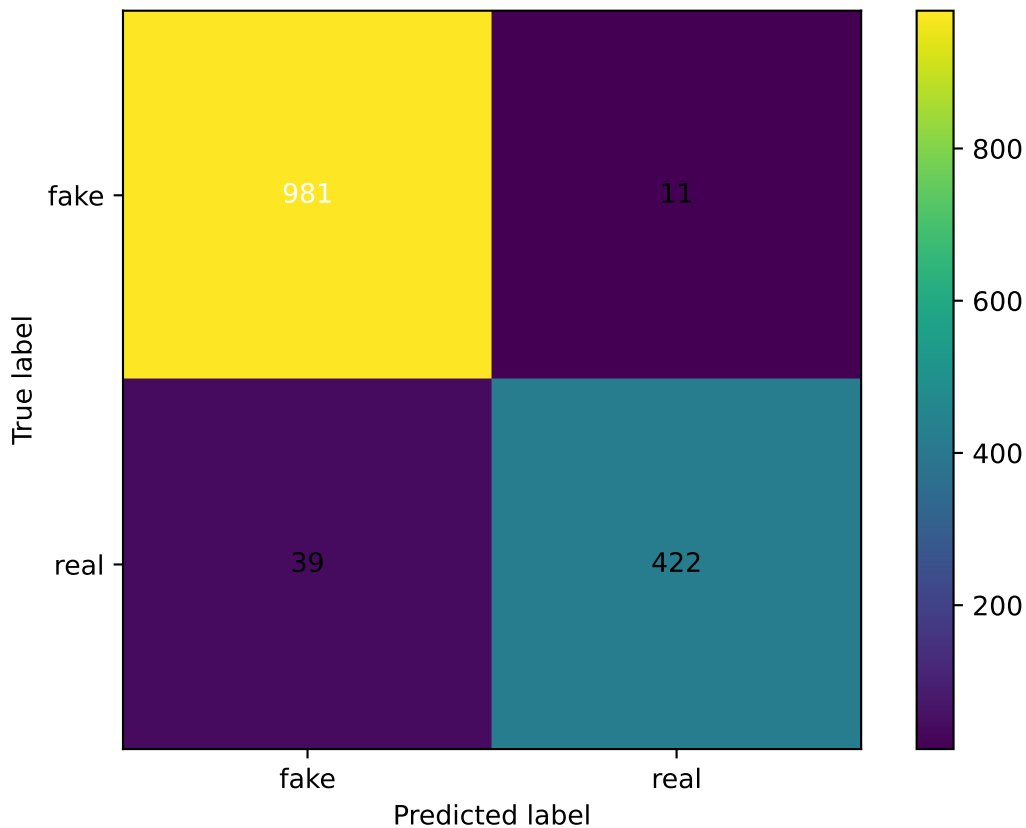
ONNX Confusion Matrix
