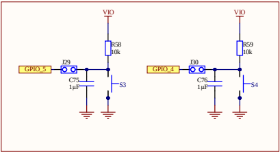
User configurable switches
