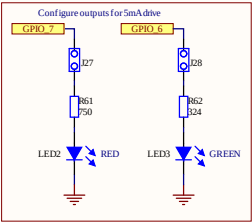
User configurable LEDs
