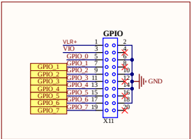
GPIO IDE Connector
