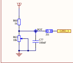
User configurable potentiometer
