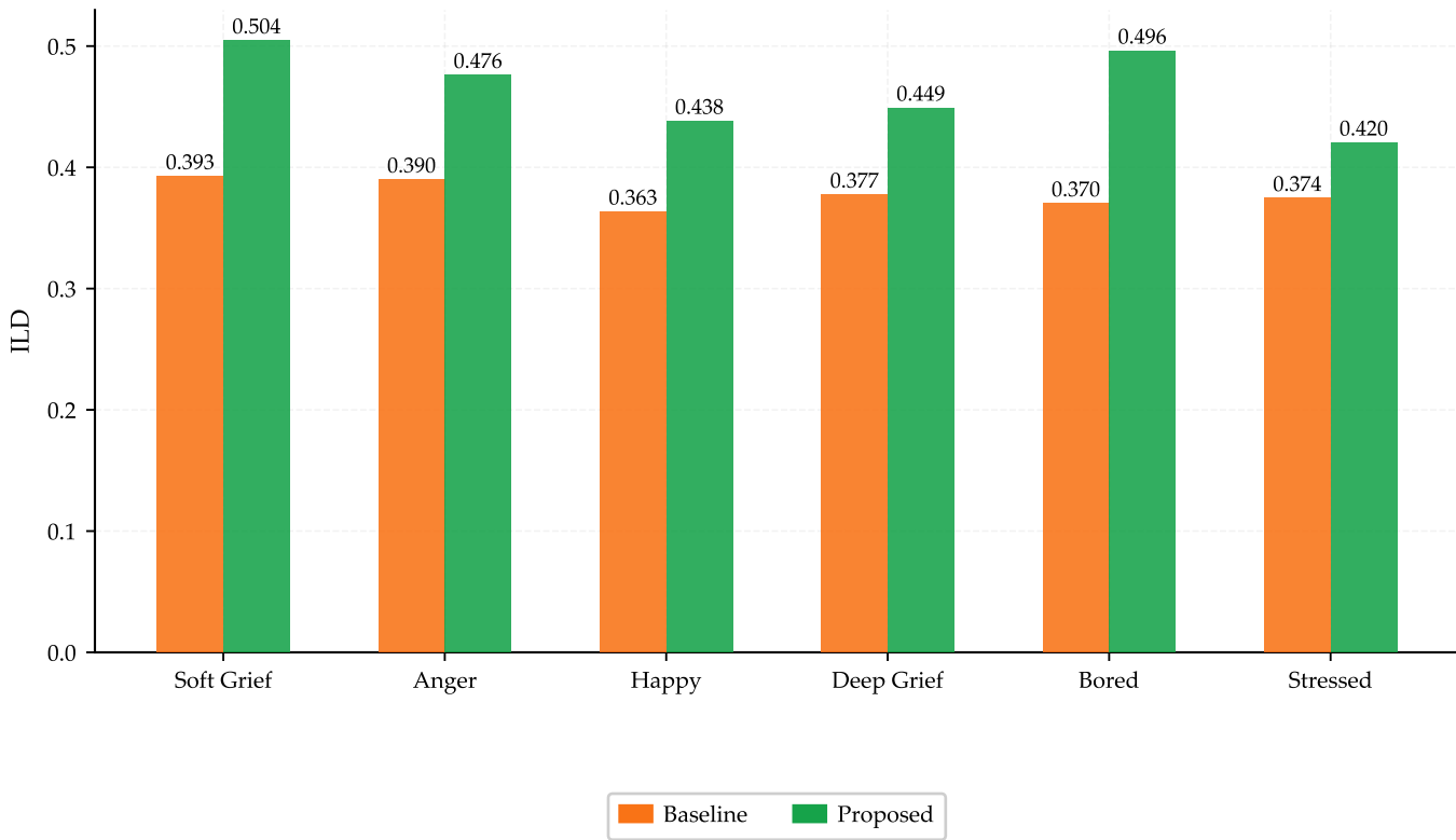
Emotion-Aware Chatbot — Diversity Comparison
