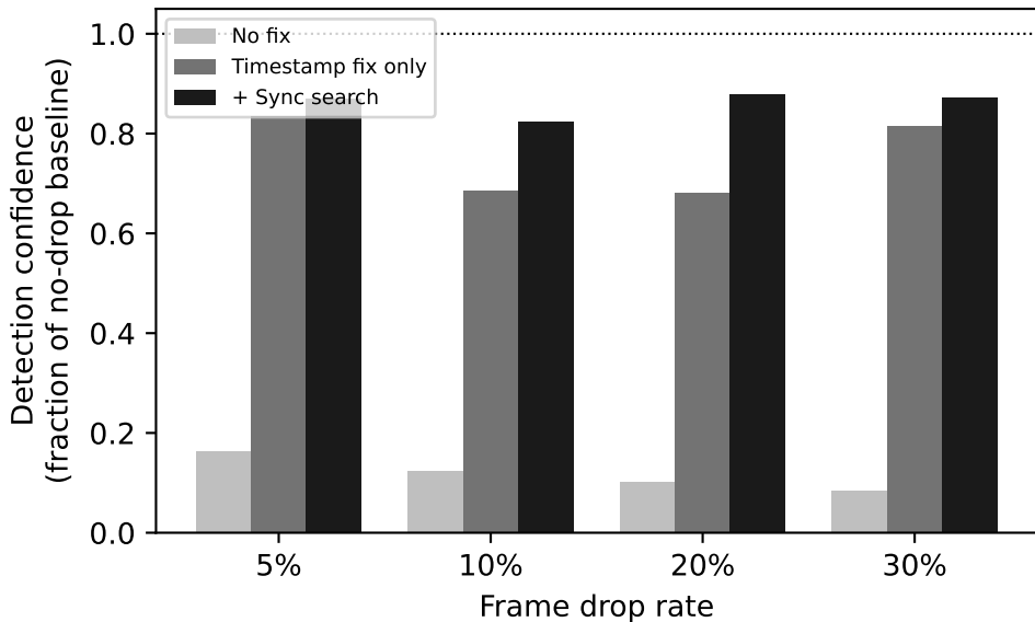
Frame-drop recovery: mean over 20 videos
