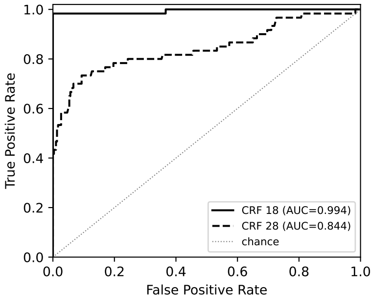
ROC: H.264 CRF 18 vs. CRF 28 (H0 pooled, n=300)
