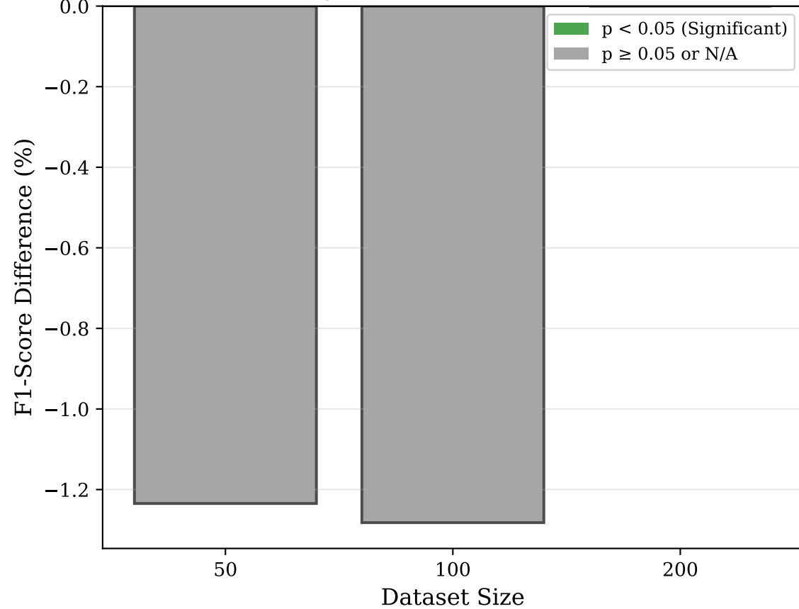
(b) Statistical Significance of Performance Difference
