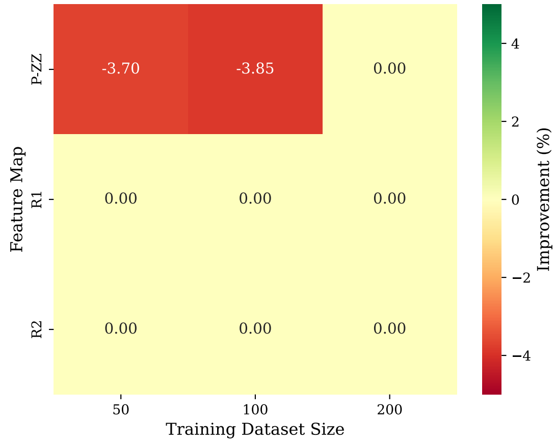
(a) F1-Score Improvement over Classical (%)
