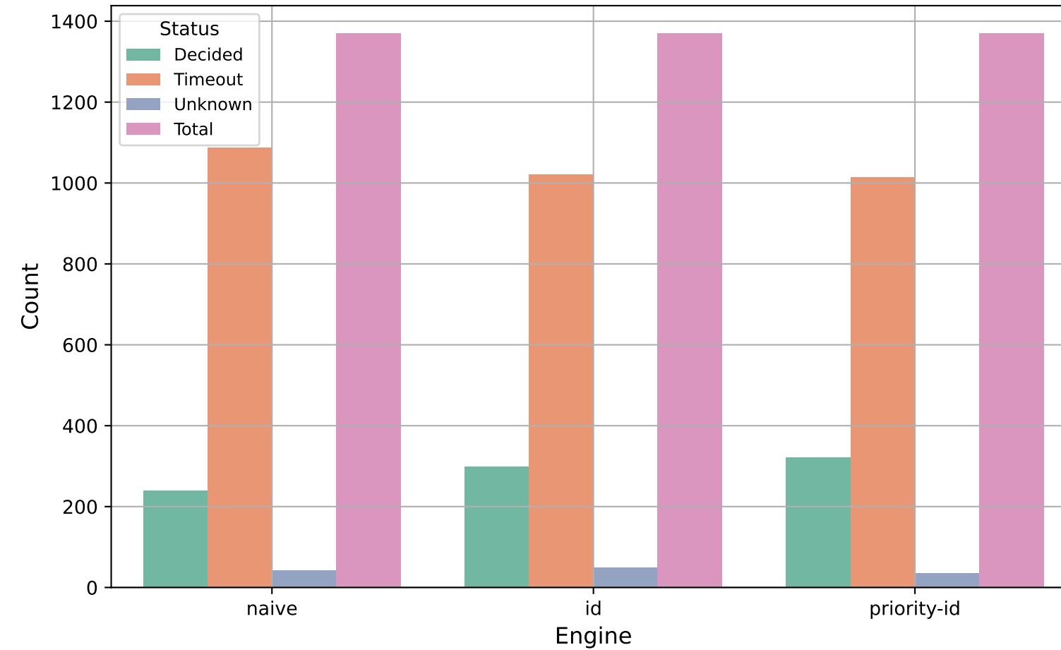
Decided vs Timeout vs Unknown
