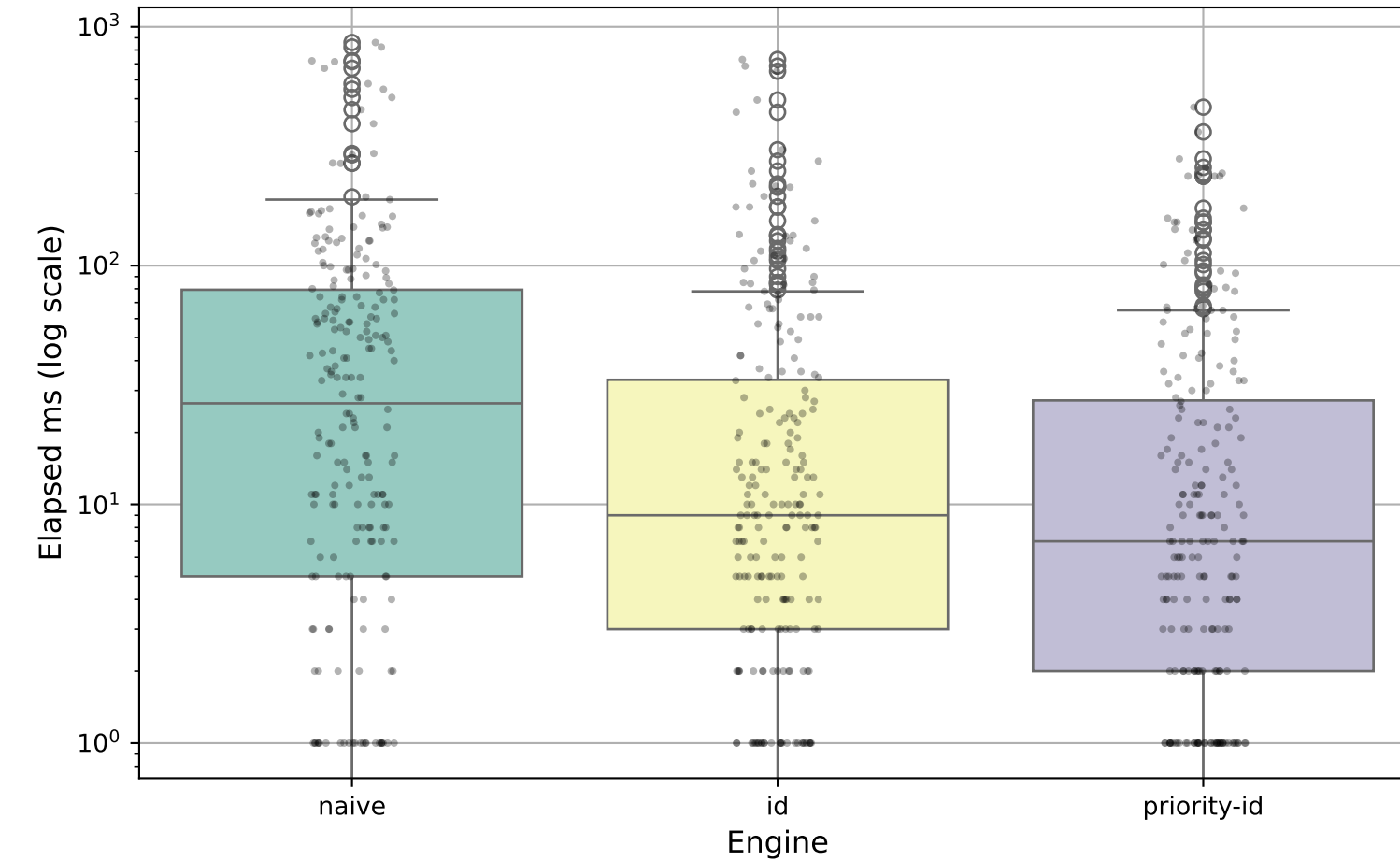
Time to Conclusion on Common Decided Problems
