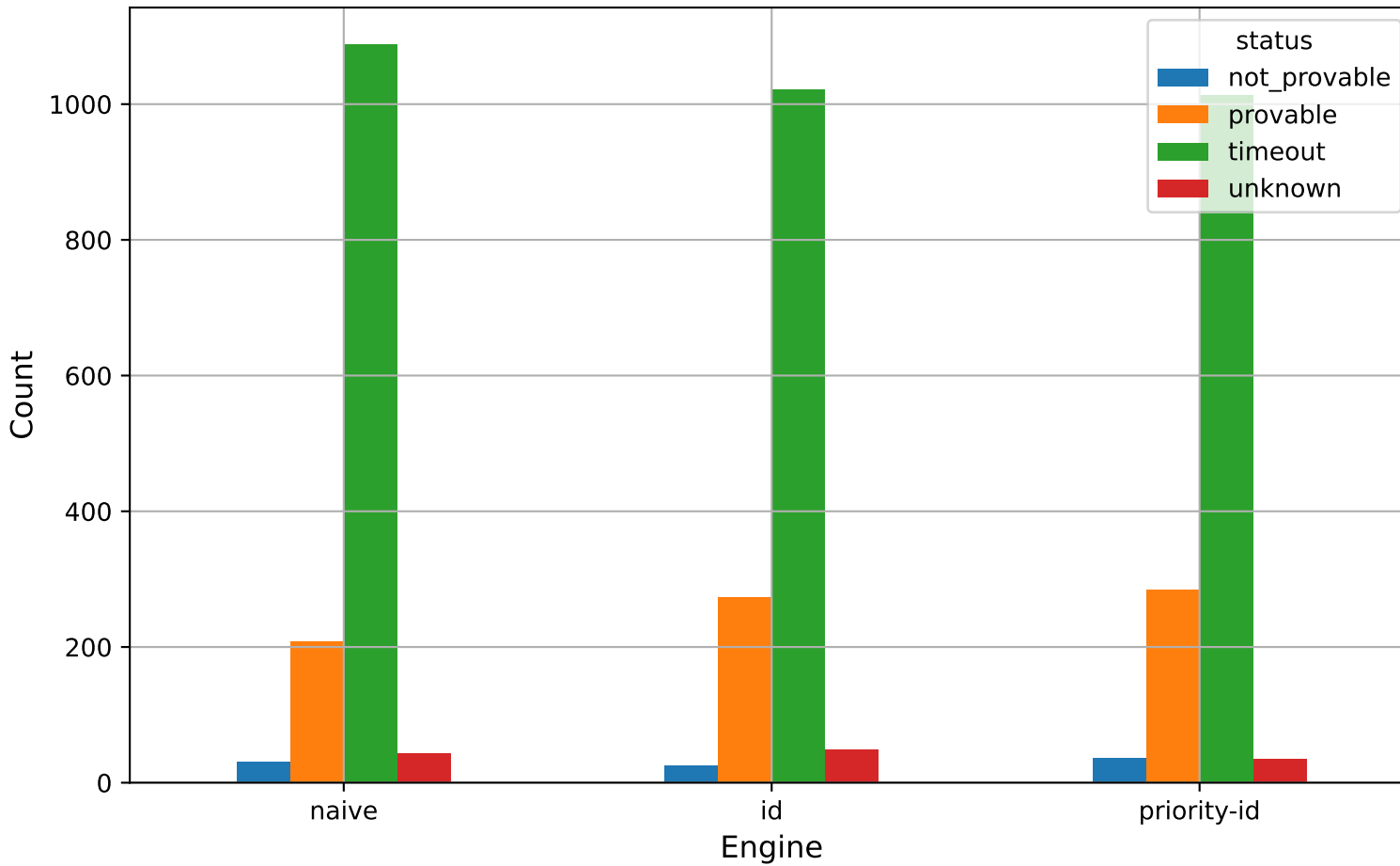
Results by Engine and Status
