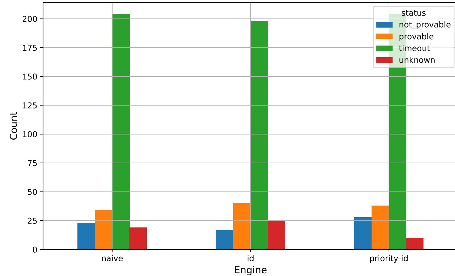
Results by Engine and Status
