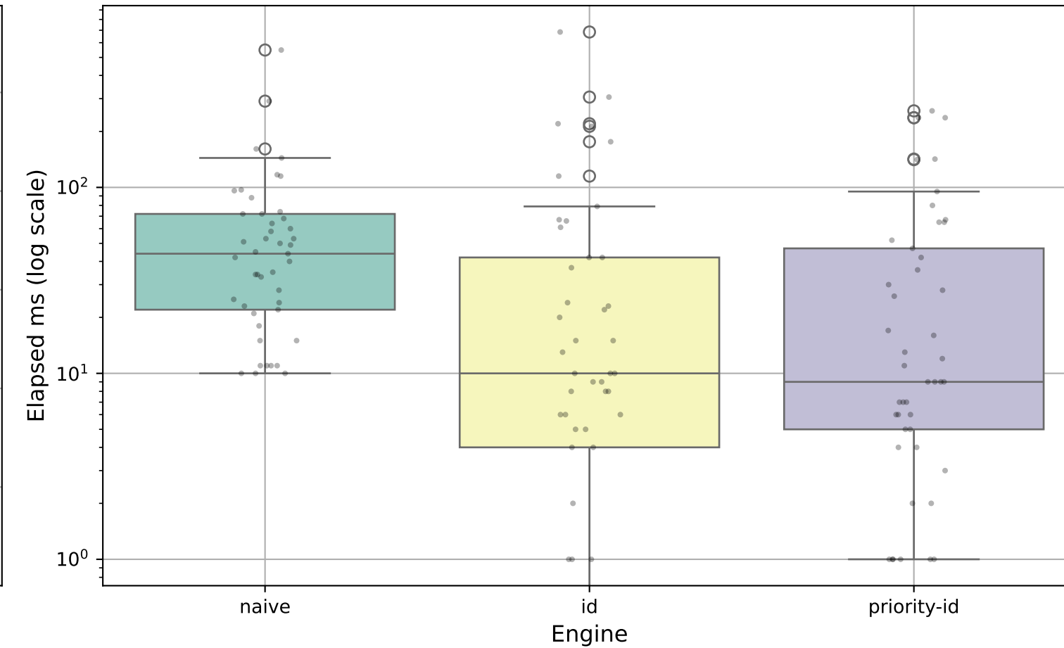
Time to Conclusion on Common Decided Problems
