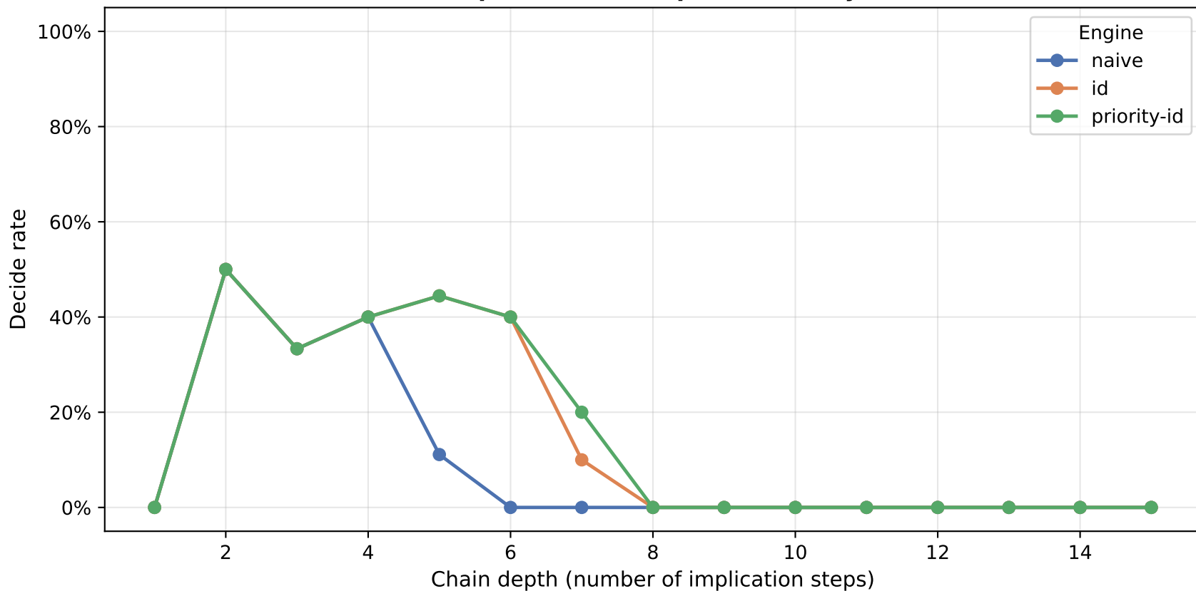
Decide Rate vs. Chain Depth (implication-chain problems only)
