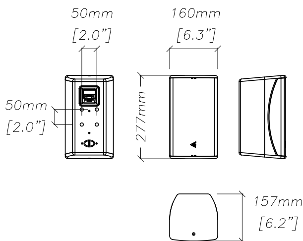
AIR-WS Wall mounting for AIR-C5
