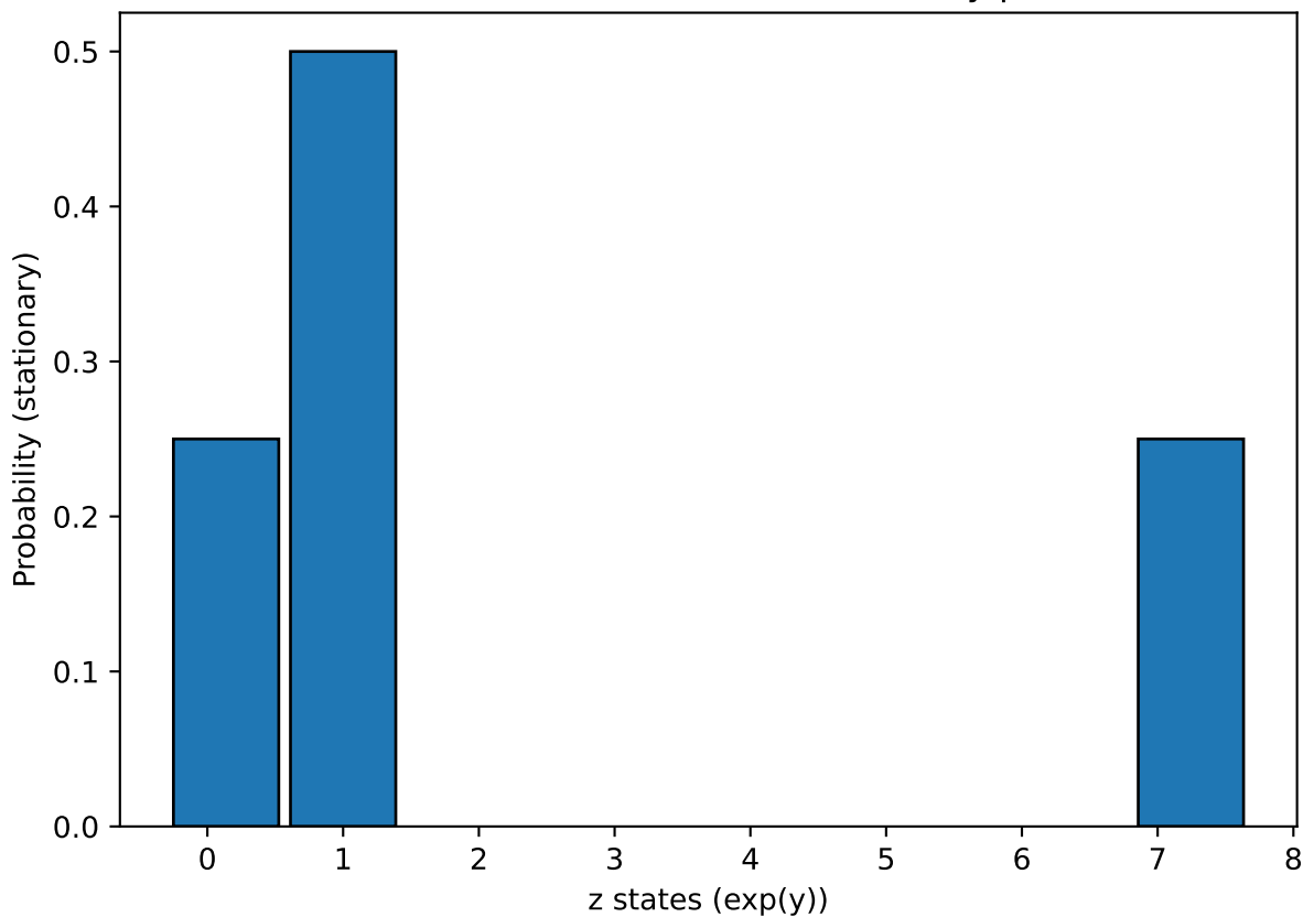
Discretized z (Rouwenhorst N=3 ): stationary probabilities
