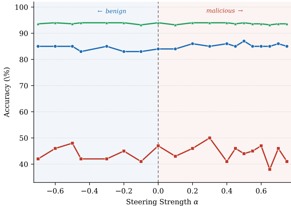
(a) Utility Benchmarks
