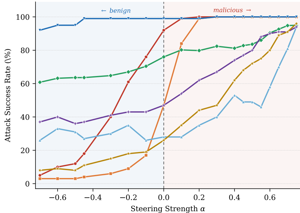
(b) Safety — Attack Success Rate
