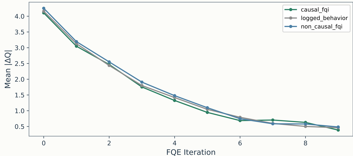
FQE Convergence: Mean Absolute Q-value Change Per Iteration
